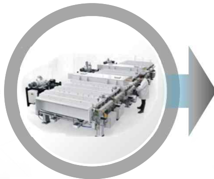
Sputtering System
