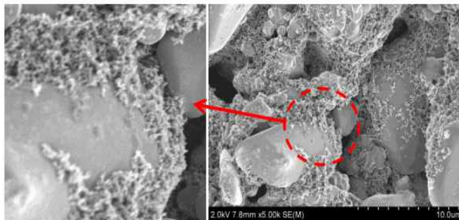
Poor Dispersed Coating with Carbon Black
