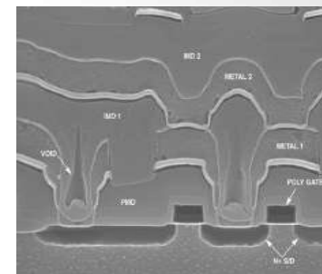
Non-planarized Integrated Circuit
