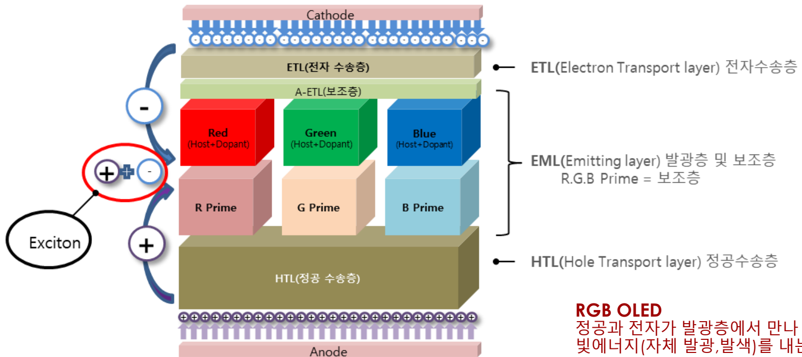
AMOLED Structure(RGB Type)
