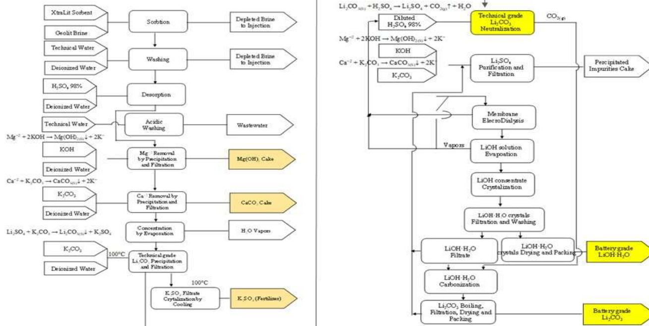
Ion Exchange DLE flow chart
