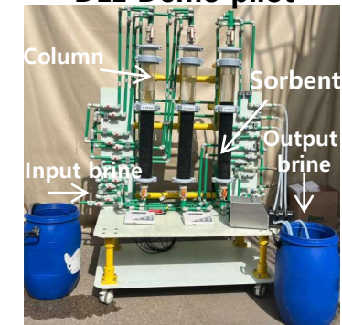
DLE Demo pilot
