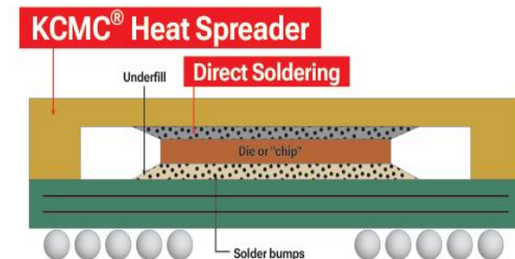
Flip-Chip Architecture
