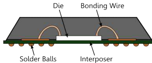
BGA Package Sideview
