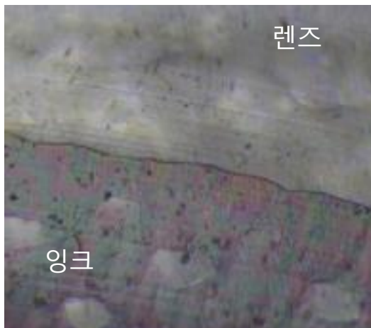
TOF-SIMS
